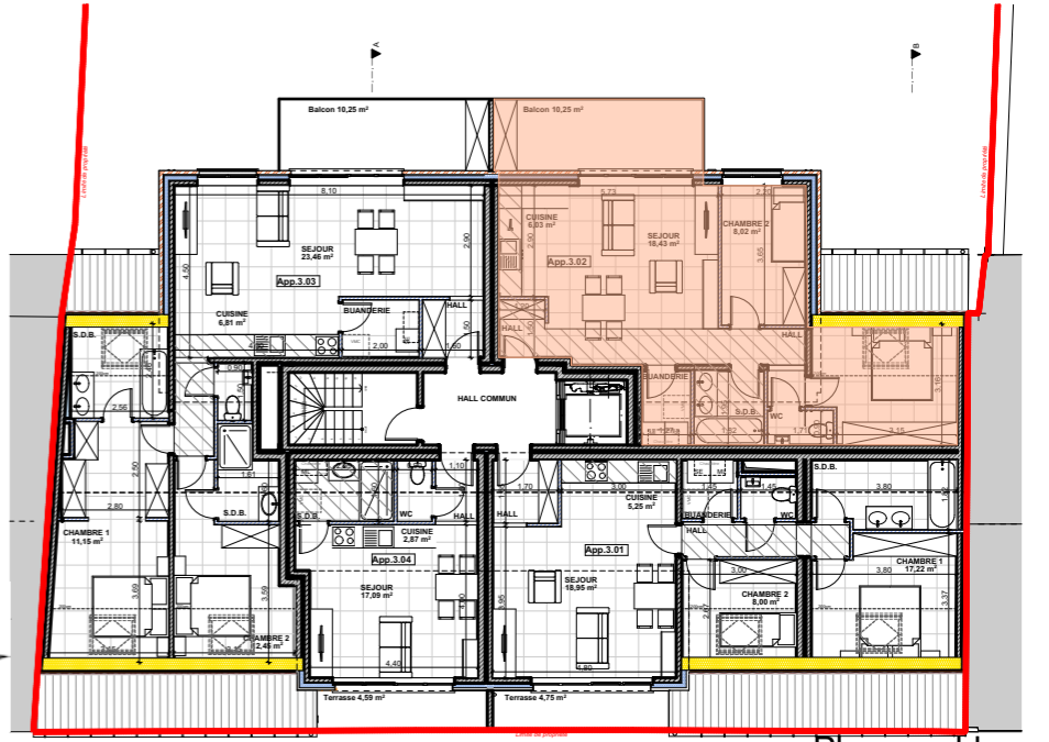
Plan combles
